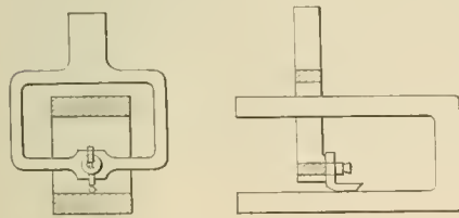
ROD PLANER TOOL.
